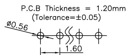
Recommended P.C.B Layout(Top Side)
