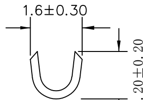
b-b SECTION
