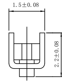
C-C SECTION
