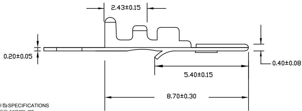
SECTION c-c
