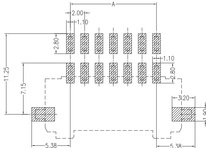
PCB LAYOUT(Tolerance:±0.05)
