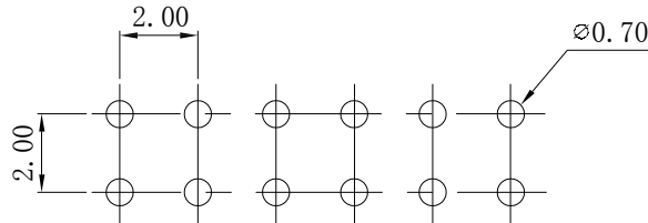
P. C. B LAYOUT
