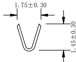
B-B SECTION
