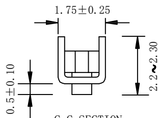
C-C SECTION
