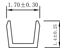
c-c SECTION
