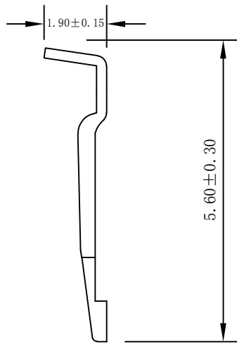
b-b SECTION
