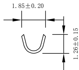
b-b SECTION
