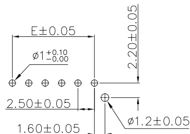
Recommended P.C.B Layout(T=1.6mm)
