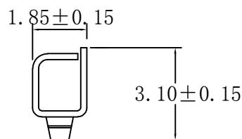
c-c SECTION
