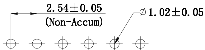
PCB LAYOUT
