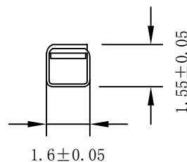
b-b SECTION
