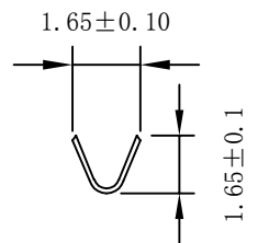
b-b SECTION
