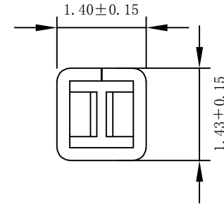
c-c SECTION
