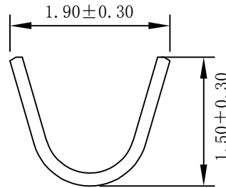
b-b SECTION
