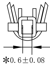
c-c SECTION
