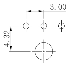
PCB. LAYOUT: 03P
