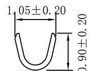
B-B SECTION
