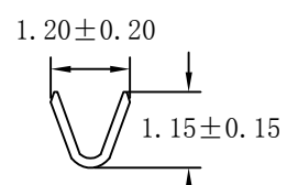
b-b section
